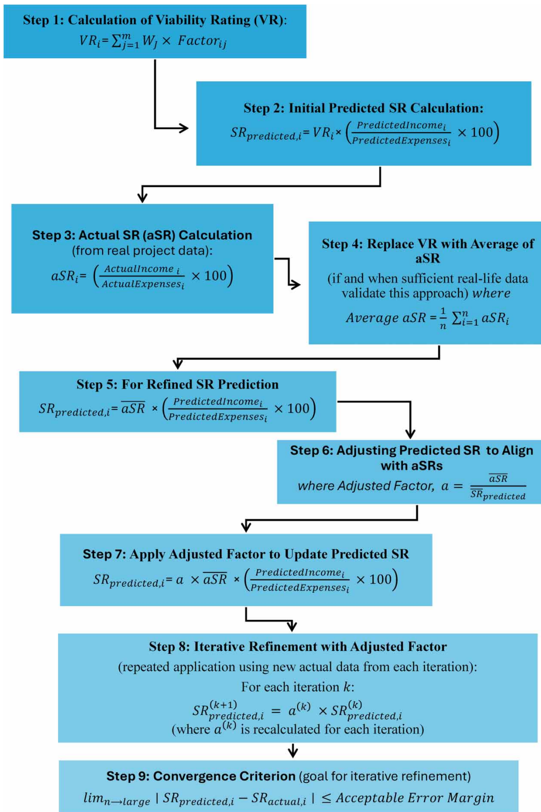
Figure 1 | Flowchart of the PISM methodology.
